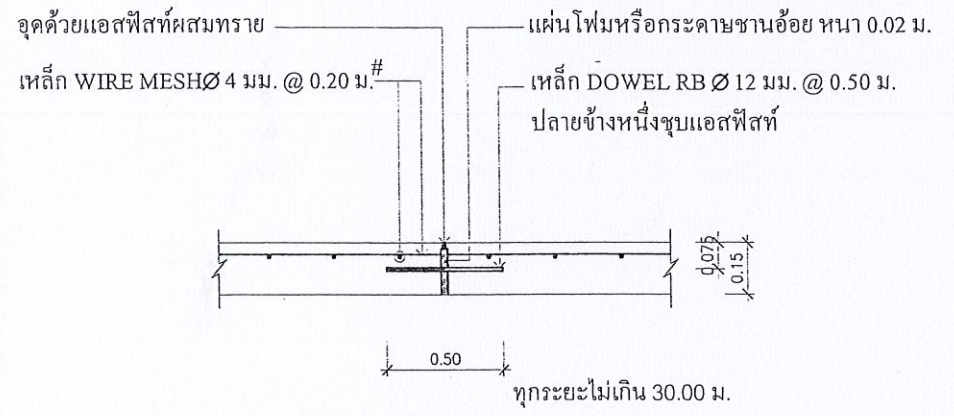
EXPANSION JOINT
