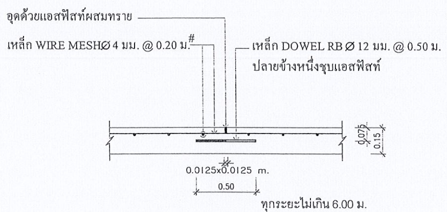
CONTRACTION JOINT
