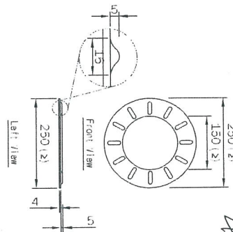
Stopper Board (GT)
