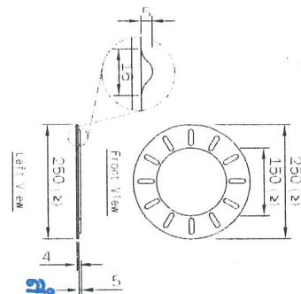
⊕ Stopper Board (GT)
